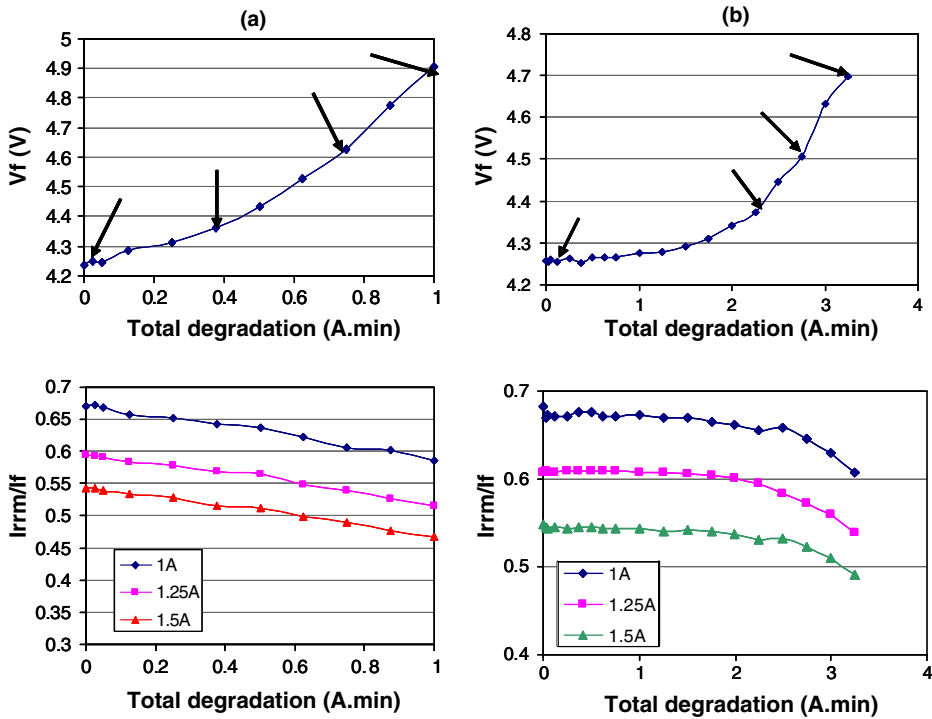
Fig. 9. The on-state voltage V_F (at 100 \text{ A/cm}^2 ) degradation and reverse recovery current for the same diodes in Fig. 8(a) and (b), respectively.
