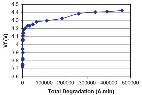
Fig. 10. On-voltage V_F (at 50 \text{ A/cm}^2 ) degradation as a function of total degradation for a 0.5 \text{ cm}^2 , 10 kV 4H-SiC PiN diode stressed at 50 A.
