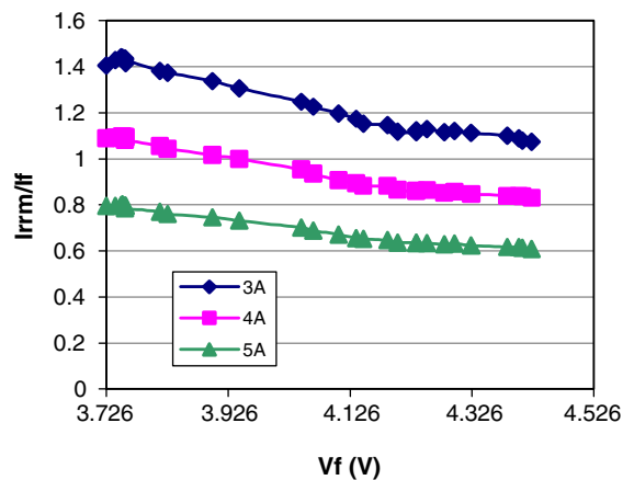
Fig. 11. Correlation between the reverse recovery peak as a function of total degradation for a 0.5 \text{ cm}^2 , 10 kV 4H-SiC PiN diode.
