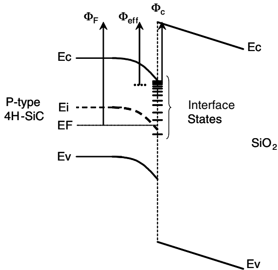
Fig. 2. SiC MOSFET under weak inversion case. The relevant barrier heights for FN tunneling in SiC-SiO 2 interface: \Phi_c is the conduction band offset, \Phi_F is the theoretical FN barrier height, and \Phi_{eff} is the effective barrier height due to the presence of interface states at the SiC-SiO 2 interface.
